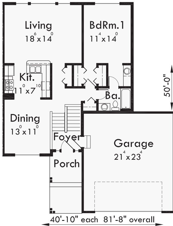
MAIN FLOOR
