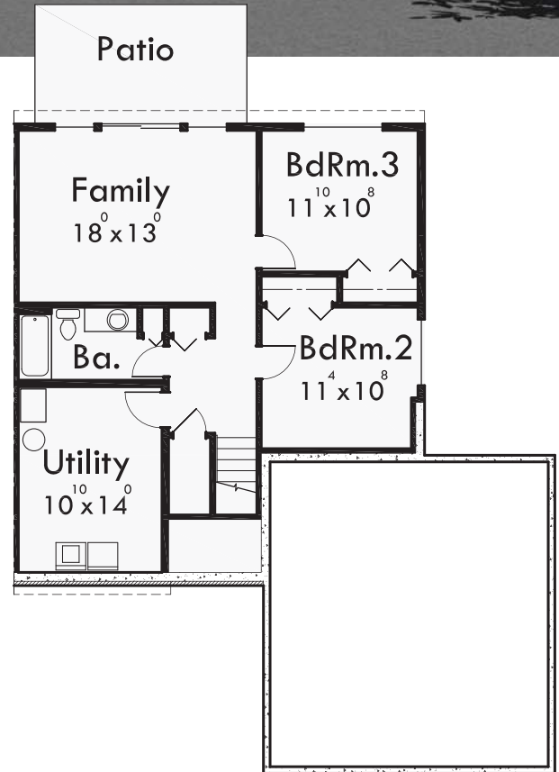
LOWER FLOOR
