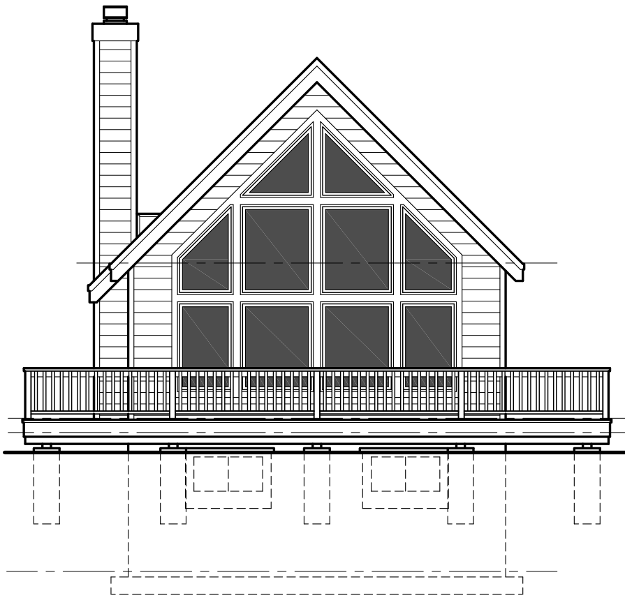
FRONT ELEVATION
