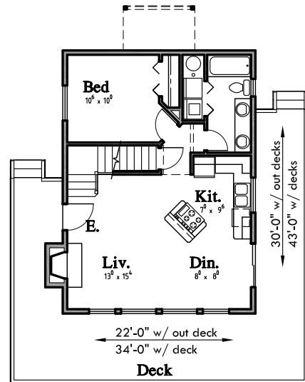
MAIN FLOOR
