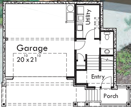
LOWER FLOOR PLAN
